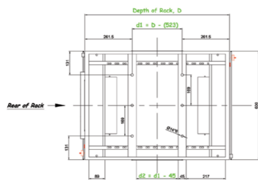
SSR 600 - Bottom View
