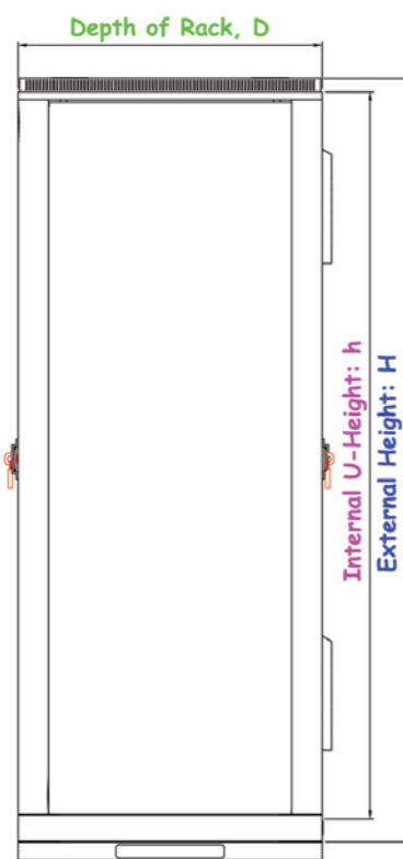
SSR W600 - Side View
