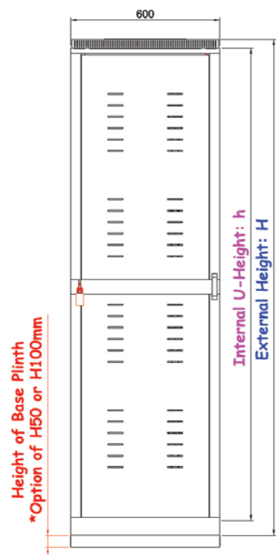
SSR W600 - Front View
