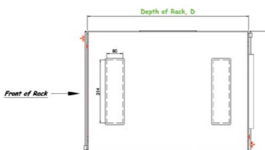
SSR 600 - Plan View
