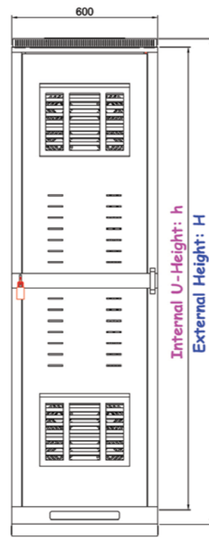
SSR W600 - Rear View with Optional Welded Fan Canopy
